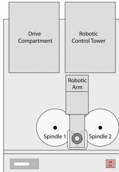
Figure 1-3 Robotic Duplicator (100 Capacity) Top View
